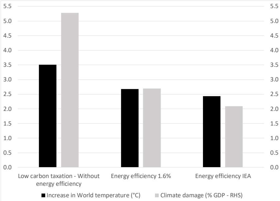
Graph 1: 2100 increase in world temperature and climate damage in LCT scenario with or without faster energy efficiency gains
