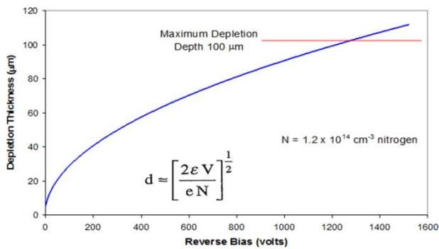
Fig. 3. Depletion depth as a function of applied reverse bias for a 100- \mu\text{m} thick epitaxial layer with a nitrogen concentration of 1.2 \times 10^{14} \text{ cm}^{-3} . The maximum depletion depth (horizontal red line) is the thickness of the epitaxial layer. A reverse bias of 1200 v is required for full depletion. If the reverse bias is limited to 1000 v, a 90- \mu\text{m} depletion depth results.
