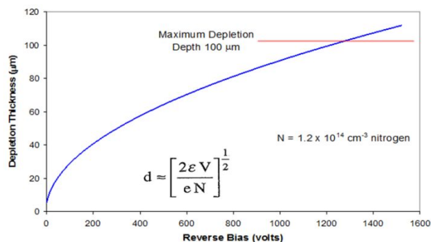
Fig. 3. Depletion depth as a function of applied reverse bias for a 100- \mu\text{m} thick epitaxial layer with a nitrogen concentration of 1.2 \times 10^{14} \text{ cm}^{-3} . The maximum depletion depth (horizontal red line) is the thickness of the epitaxial layer. A reverse bias of 1200 v is required for full depletion. If the reverse bias is limited to 1000 v, a 90- \mu\text{m} depletion depth results.
