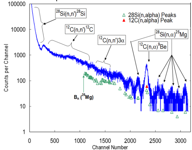
Fig. 7. Response spectrum for a 6 \text{mm}^2 \times 100 \mu\text{m} SiC detector exposed to 14.1 MeV DT neutrons. (Reproduced from Reference 25)
