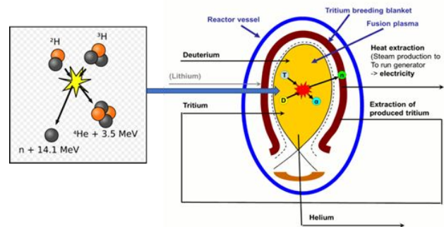
16. Schematic representation of a Tokamak nuclear fusion reactor.
