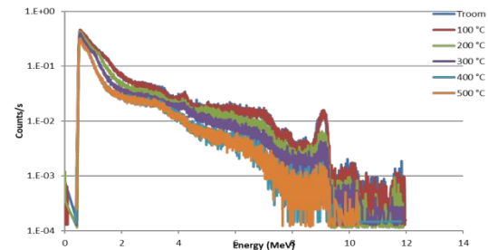
Fig. 9. Energy spectra recorded during irradiation tests of SiC-based detectors with 14 MeV neutrons at different ambient temperatures. (Figure reproduced from reference 40).
