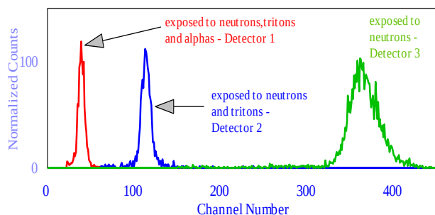
Fig. 11. Comparison of the ^{238}\text{Pu} pulse-height response of three detector configurations following irradiation. (Figure reproduced from Reference 55)
