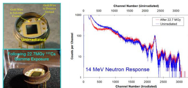
Fig. 10. Photographs of a 6-mm 2 x 100- \mu\text{m} SiC Schottky diode before (top) and after (bottom) exposure to a cumulative ^{137}\text{Cs} gamma-ray dose of 22.7 MGy and comparison of the corresponding neutron responses (Figures adapted from reference 48)
