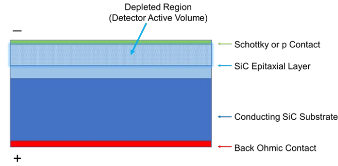
Fig. 2 Application of a reverse bias forms a depletion region in the epitaxial layer which corresponds to the active volume of the detector
