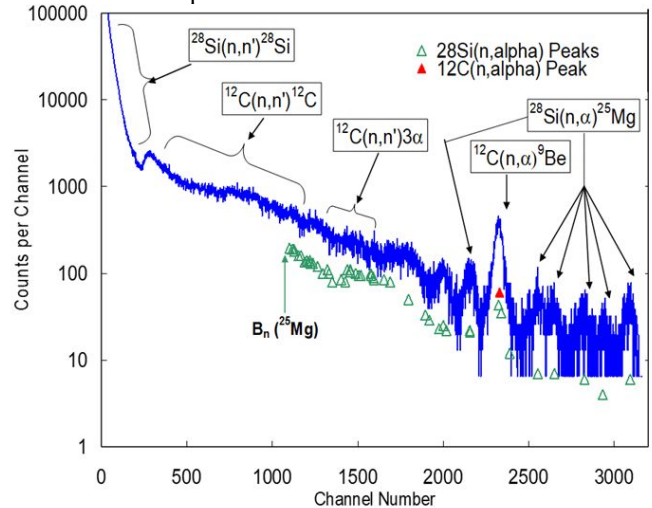
Fig. 7. Response spectrum for a 6 mm ^2 \times 100 \mu\text{m} SiC detector exposed to 14.1 MeV DT neutrons. (Reproduced from Reference 25)
