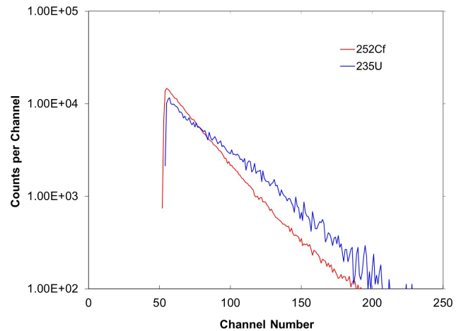
Fig. 6. Comparison of the response spectra of a SiC detector to neutron-induced fission neutrons from ^{235}\text{U} and ^{252}\text{Cf} spontaneous fission neutrons. (Adapted from Reference 36)
