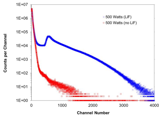
Fig. 4. Comparison of the neutron response of a 500- \mu\text{m} diameter \times 3- \mu\text{m} SiC Schottky diode to reactor fission neutrons with and without a 24.2- \mu\text{m} ^6\text{LiF} converter foil. With the ^6\text{LiF} foil present, the detector response is primarily to thermal neutrons. When the ^6\text{LiF} foil is absent, the detector responds primarily to fast neutrons. (Figure reproduced from Reference 32).
