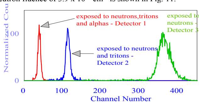
Fig. 11. Comparison of the ^{238}\text{Pu} pulse-height response of three detector configurations following irradiation. (Figure reproduced from Reference 55)
