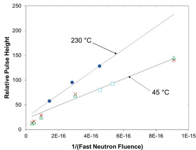
Fig. 14. Effect of elevated temperature during neutron irradiation on the observed pulse heights from a 238 Pu alpha test source. Pulse height is plotted as a function of reciprocal fast neutron fluence. The symbols refer to different irradiated SiC detectors. (Figure adapted from Reference 55)
