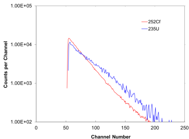
Fig. 6. Comparison of the response spectra of a SiC detector to neutron-induced fission neutrons from ^{235}\text{U} and ^{252}\text{Cf} spontaneous fission neutrons. (Adapted from Reference 36)
