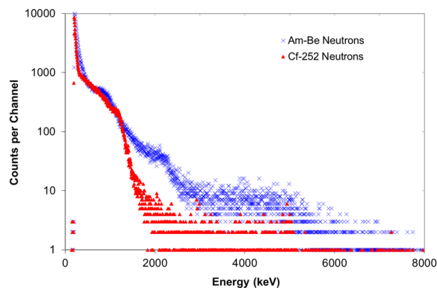
Fig. 5. Comparison of the responses of a SiC detector to fission neutrons from ^{252}\text{Cf} and neutrons from an ^{241}\text{Am} -beryllium source. (Adapted from reference 25)
