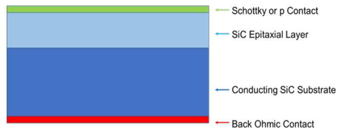
Fig. 1. Schematic representation of a SiC epitaxial diode detector structure.
