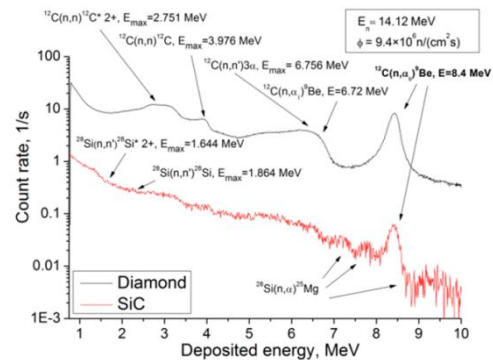
Fig. 8. Comparison of the responses of SiC-based and CVD diamond-based detectors to 14.12 MeV neutrons. (Figure reproduced from Reference [38].)
