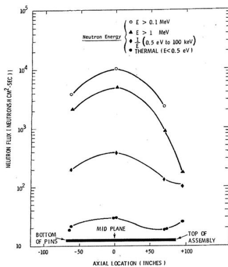
Fig. 15 Axial neutron fluence rate distributions for a typical PWR spent-fuel assembly (Figure reproduced from Reference [59].
