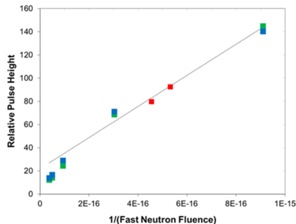
Fig. 12 ^{238}\text{Pu} pulse heights for SiC diodes exposed to fast neutrons. Pulse height is plotted as a function of reciprocal fast-neutron fluence. (Figure reproduced from Reference [55])
