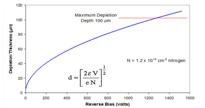
Fig. 3. Depletion depth as a function of applied reverse bias for a 100-μm thick epitaxial layer with a nitrogen concentration of 1.2 \times 10^{14} \text{ cm}^{-3} . The maximum depletion depth (horizontal red line) is the thickness of the epitaxial layer. A reverse bias of 1200 v is required for full depletion. If the reverse bias is limited to 1000 v, a 90-μm depletion depth results.
