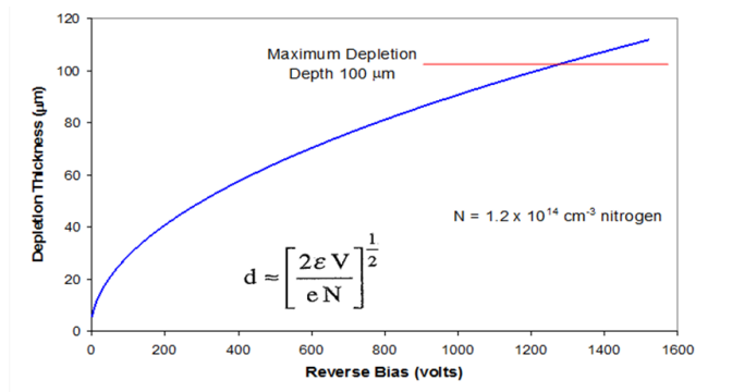
Fig. 3. Depletion depth as a function of applied reverse bias for a 100-μm thick epitaxial layer with a nitrogen concentration of 1.2 \times 10^{14} \text{ cm}^{-3} . The maximum depletion depth (horizontal red line) is the thickness of the epitaxial layer. A reverse bias of 1200 v is required for full depletion. If the reverse bias is limited to 1000 v, a 90-μm depletion depth results.
