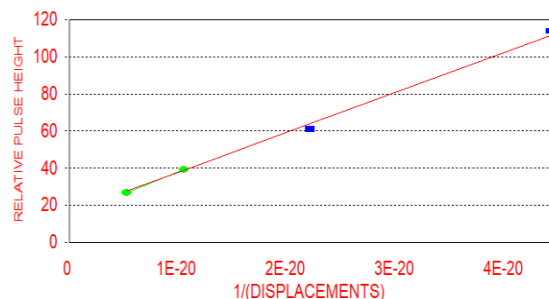
Fig. 13 ^{238}\text{Pu} pulse heights for SiC diodes exposed to fast neutrons and neutron reaction-product ions. Pulse height is plotted as a function of reciprocal calculated displacements. The ovals correspond to neutron plus triton plus alpha-particle exposures and the squares correspond to neutron plus triton exposures (Figure reproduced from Reference [55])
