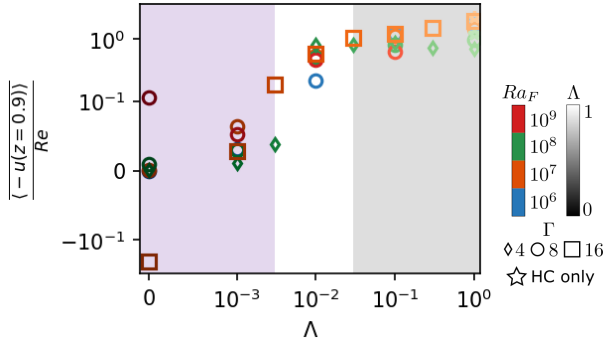
Figure 9: Temporally- and horizontally-averaged horizontal flow near the top boundary at z = 0.9 normalized by the Reynolds number as a function of \Lambda . \langle -u(z = 0.9) \rangle_x is of the same order as Re for relatively large \Lambda .
