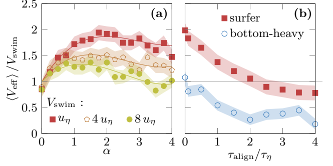
FIG. 4. (a) Performance ( V_{\text{eff}}/V_{\text{swim}} ) of surfers using a time dependent \tau as a function of the dimensionless constant \alpha (Eq. (8)) for different swimming velocities V_{\text{swim}} . Solid lines represent a fit with Chebyshev polynomials of degree 3. (b) V_{\text{eff}}/V_{\text{swim}} of surfers and bottom-heavy swimmers as a function of the reorientation time \tau_{\text{align}} . V_{\text{swim}} = u_\eta . Shaded area represents the 95% confidence interval.
