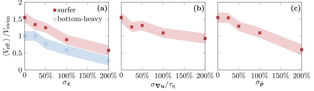
FIG. S4. Robustness of the surfing strategy. Performance as a function of noise intensity on: (a) the measure of \hat{\mathbf{z}} , (b) the flow velocity gradients \nabla \mathbf{u} sensing, (c) the control of the swimming direction \hat{\mathbf{p}} . The noise is modeled as a Gaussian white noise of standard deviation \sigma . The shaded area represents the 95% confidence interval. Parameters: V_{\text{swim}} = 4u_{\eta} and \tau_{\text{align}} = 0 .
