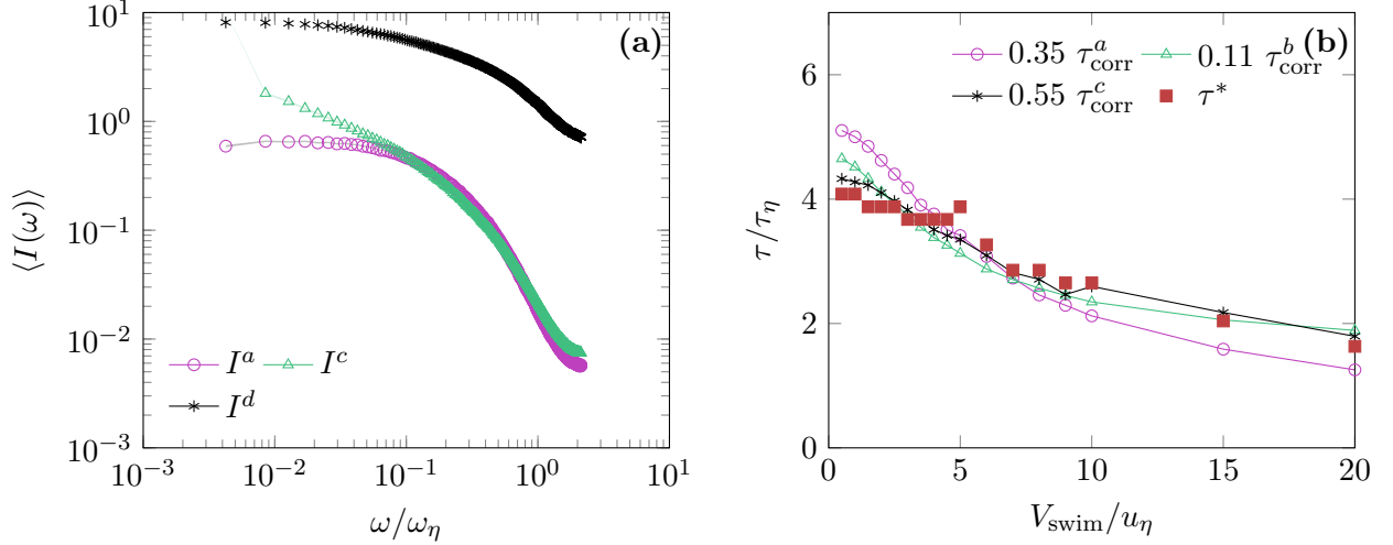
FIG. S3. Correlation time dependence on the choice of the gradients invariant. (a) I(\omega) , module of the temporal Fourier transform of various invariants of the velocity gradients (defined in Tab. I), measured along trajectories of bottom-heavy swimmers ( \hat{n} = \hat{p} = \hat{z} ) for various swimming speeds. \omega_\eta = 2\pi/\tau_\eta . The shaded area represents the 95% confidence interval. (b) Correlation time \tau_{\text{corr}} (Eq. (S11)) and optimal time horizon \tau^* as a function of swimming velocity.
