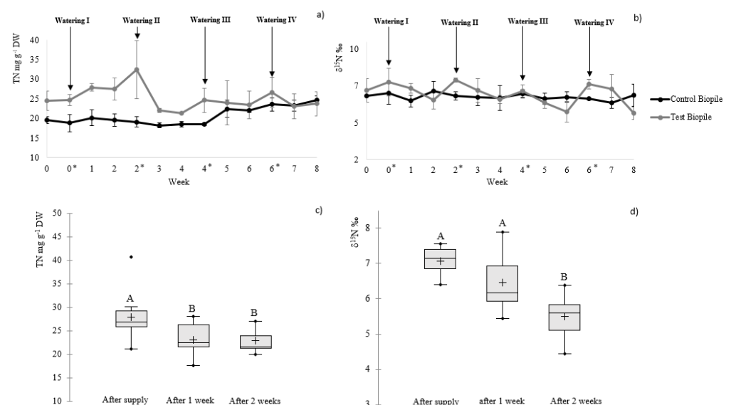
Figure 3. (a) Temporal evolution of the total nitrogen (TN) concentration; (b) temporal evolution of the isotopic signature ( \delta^{15}\text{N} ) (* means after watering, and the error bars represent standard deviations ( n = 3 )); (c) monitoring of the total nitrogen (TN) abatement evolution in the test biopile; and (d) the isotopic signature ( \delta^{15}\text{N} ) ( n = 3 ) evolution in the test biopile. Different letters above boxplots indicate a significant difference between plots according to the Kruskal–Wallis test with Dunn’s procedure, (a–c) p value = 0.05, (d) p value = 0.001.
