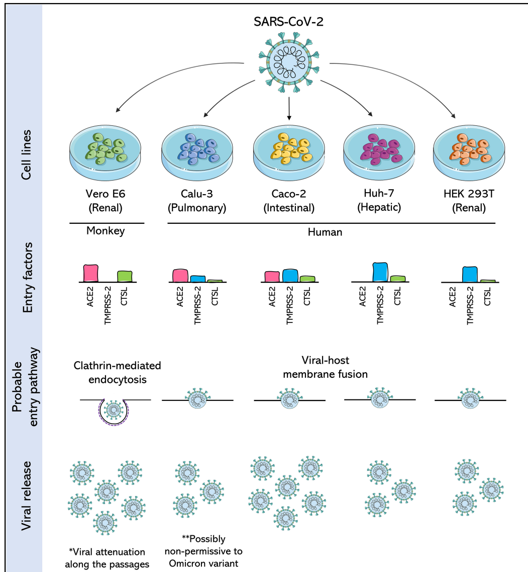
FIGURE 2 Comparison of SARS-CoV-2 permissive cell lines. Four human cell lines: Calu-3 (Pulmonary), Caco-2 (Intestinal), Huh-7 (Hepatic) and HEK 293T (Renal), are compared with each other and with the Vero E6 cell, a cell derived from the African green monkey kidney, and widely used in the isolation and production of SARS-CoV-2. Cells are compared for the expression of three important entry factors used by SARS-CoV-2: angiotensin-converting enzyme 2 receptor (ACE2), transmembrane protease serine 2 (TMPRSS2) and the lysosomal protease cathepsin L (CTSL), based on data from Murgolo et al., 2021; Saccon et al., 2021 and Shuai et al., 2020. The expression of these factors dictates the entry pathway used by SARS-CoV-2. The release of SARS-CoV-2 viral particles is also compared. The asterisks draw attention to likely consequences of producing SARS-CoV-2 in these cells.
