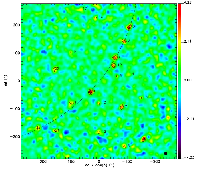
Fig. 1. GJ526 field, mapped with NIKA2 in the 1.15-mm continuum waveband (colour scale: \text{mJy beam}^{-1} , contours: S/N). Source IDs are those in Table 1. The curve traces the filament-like structure identified across the map. S/N contours are -3, +3, +4, +5, +6, \dots (the negative contours are dashed white lines and can be seen better when the map is zoomed in the electronic version. The S/N = -4 level was processed in plotting the map but no such negative feature was apparent. For the noise rms per pixel, we refer the reader to Fig. 5. Pixel size is 2 arcsec. J2000 coordinates of the map centre are 13\text{h}45\text{m}44.52\text{s} and +14^\circ53'20.6'' . The filled black circle in the bottom right corner shows the HPBW.
