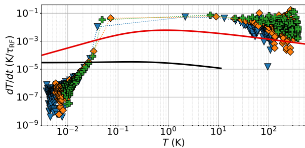
FIG. 3. Log-log representation of dT/dt vs temperature in a time-scale in units of the rf period \tau_{RF} . Colored symbols : free evolution of N ions and a rf trapping potential characterised by q_x = 0.6 . Blue triangles : N = 256 , Orange diamonds : N = 512 , Green crosses : N = 1024 (the dotted lines are guide to the eyes). Red solid lines : cooling rate G as defined by Eq. (6) for detuning \delta_L = -\Gamma . Black line : spontaneous emission induced heating H_e as defined by Eq. (7) for \delta_L = -\Gamma .
