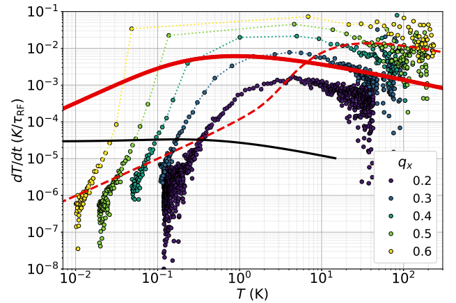
FIG. 2. Log-log representation of dT/dt vs temperature in a time-scale in units of the rf period \tau_{RF} . Coloured symbols : free evolution H of an ensemble of 1024 ions in an rf trapping potential characterised by q_x = 0.2, 0.3, 0.4, 0.5, 0.6 (see the colour chart, the dotted lines are guide to the eyes). Red lines : cooling rates G as defined by Eq. (6) for different laser detuning : solid line : \delta_L = -\Gamma , dashed line : \delta_L = -10\Gamma . Black line : spontaneous emission induced heating H_e as defined by Eq. (7) for \delta_L = -\Gamma .
