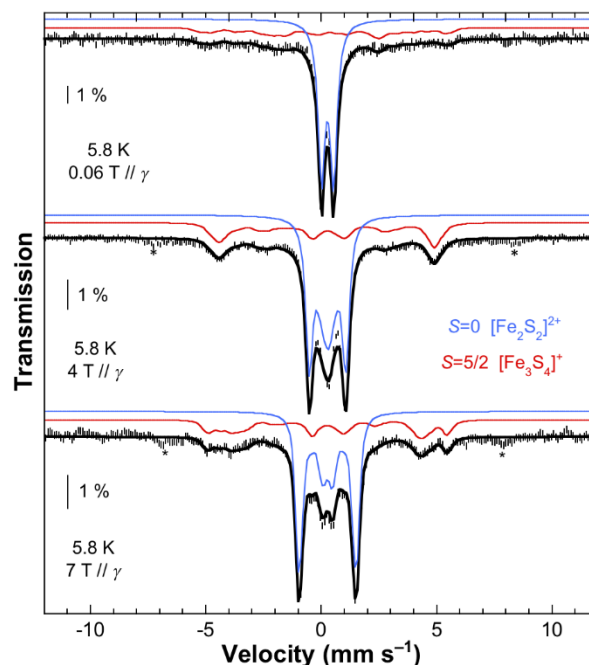
Figure 4. Mössbauer spectra of mimivirus air-purified recombinant GciS showing the signatures of S=0 [2Fe-2S] 2+ and S=5/2 linear [3Fe-4S] 1+ clusters. The black line is the spectral simulation resulting from the addition of individual cluster contributions.
