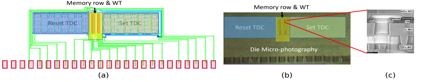
Fig. 3. (a) Layout, (b) die optical microscopy photograph of the measurement structure, with identification of the functional blocks, and (c) SEM image of the memory stack on top of the CMOS process
