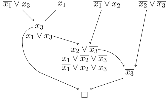
Figure 2: A max-refutation
