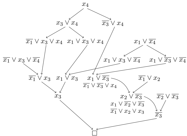
Figure 12: Adapting an unrestricted resolution refutation to a max-refutation
