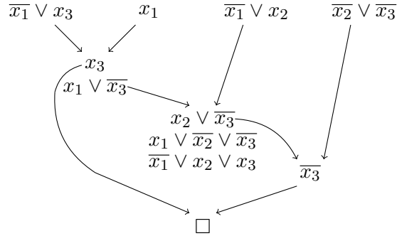
Figure 2: A max-refutation
