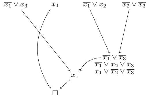
Figure 21: Second max-refutation
