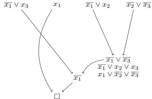
Figure 21: Second max-refutation
