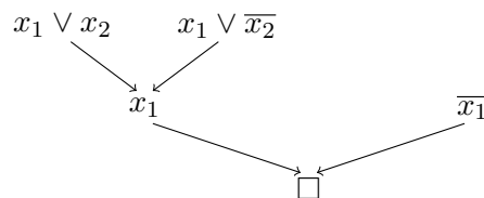
Figure 7: Regular tree-like resolution refutation after minimization
