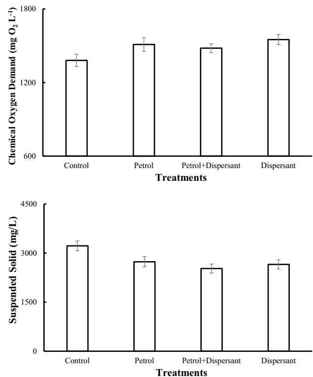
Fig. 2 Variation in COD (a) and SS (b) values after 40 days of incubation. COD is the amount of oxygen expressed in milligrams, consumed by existing materials in water and oxidizable under defined operating conditions. SS represent the solid particles responsible for the turbidity of water
