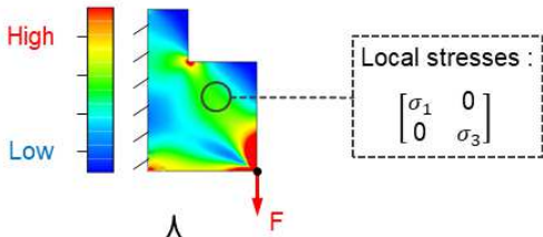
(a) Mechanical stresses in the initial part
