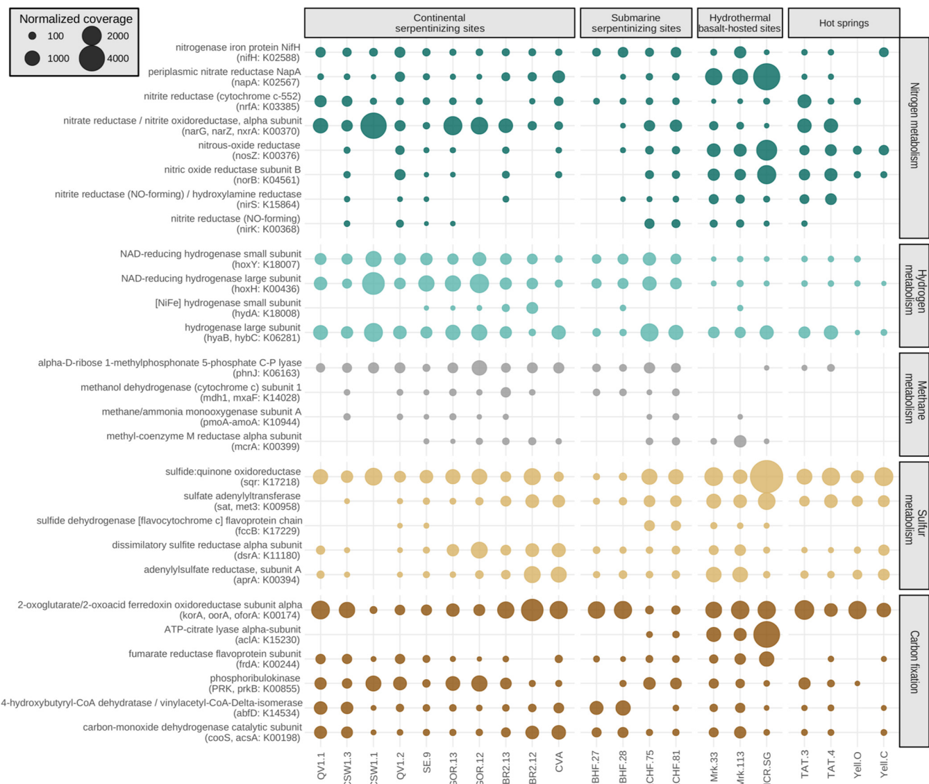
FIG 3 Potential microbial metabolisms in the 21 metagenomes from hydrothermal systems. Shown is a bubble plot of key genes involved in nitrogen (green), dihydrogen (turquoise), methane (gray), and sulfur (beige) potential metabolisms and carbon fixation (brown). The size of the circles corresponds to the abundance of normalized KOs.
