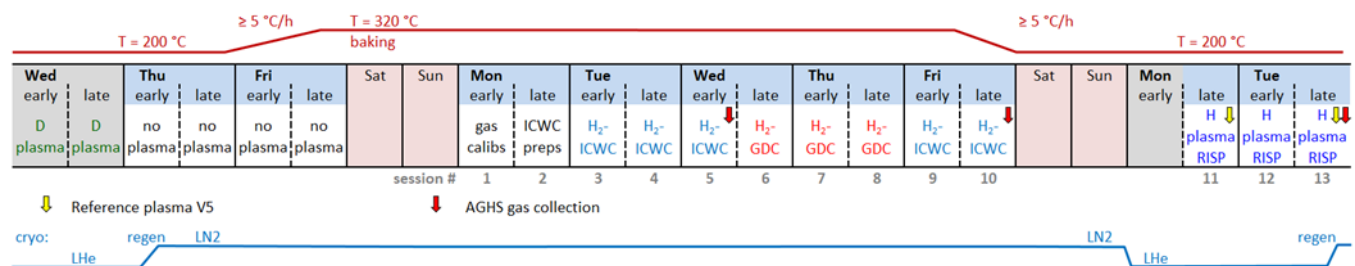
Figure 1: Timeline of the isotopic exchange experiment indicating the baking duration, the ICWC, GDC and diverted plasma operation sessions, the cooling of the divertor cryopanels, either by liquid helium or nitrogen, the collection of pumped gas at the Active Gas Handling System (AGHS) and reference pulses in the V5 divertor configuration. “Early” and “Late” refer to the two operational shifts which JET runs on each experimental day.
