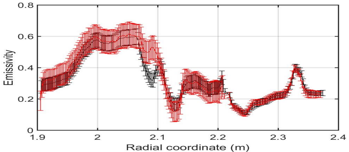
Figure 7. Emissivity distribution (black) before boronization and (red) three pulses after it, pulses #55541 and #55553, respectively.
