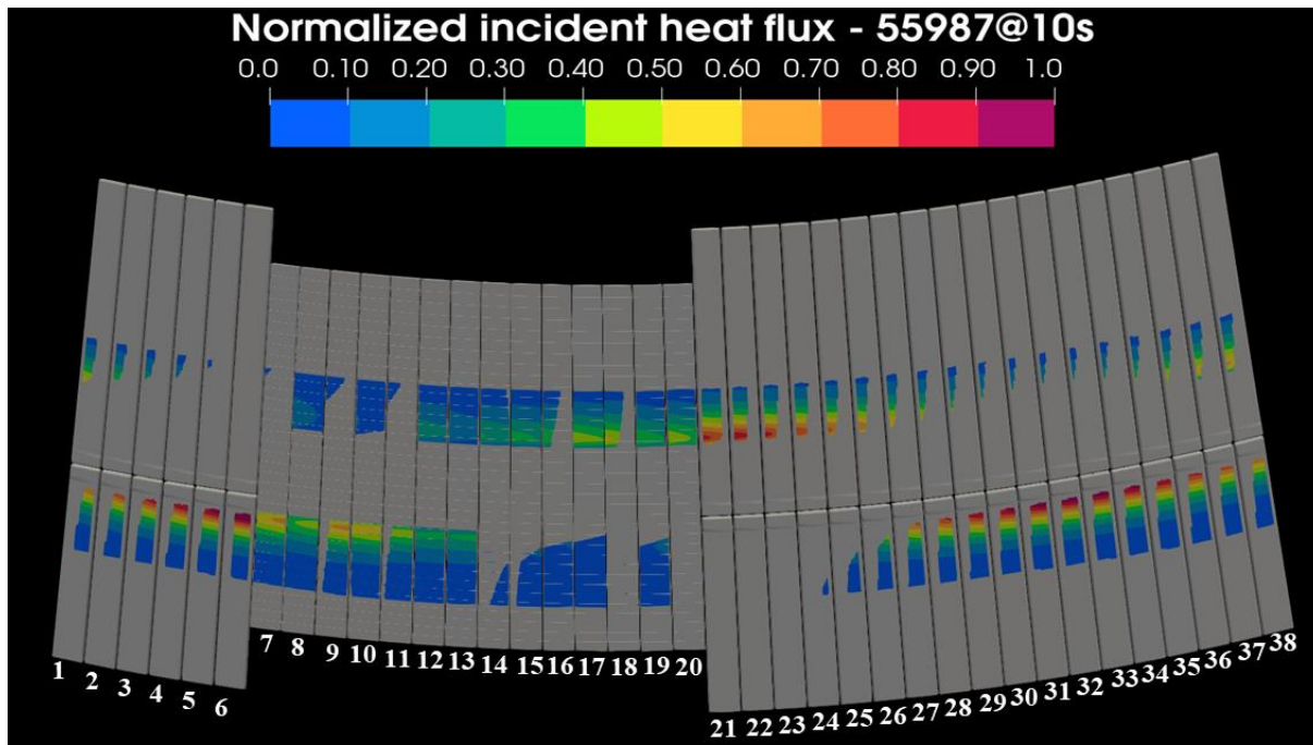
Figure 12. Normalized heat flux computed for the sector Q3B with the PFCFlux code [21] for the pulse #55987 without asymmetry and \lambda_q = 6mm [26] projected to the divertor (no spreading factor in the private flux region). The ITER-grade PFU have been moved according to the measured misalignment. The white area corresponds to the magnetic shadowed area especially visible for the PFU 14, 18 and 20.
