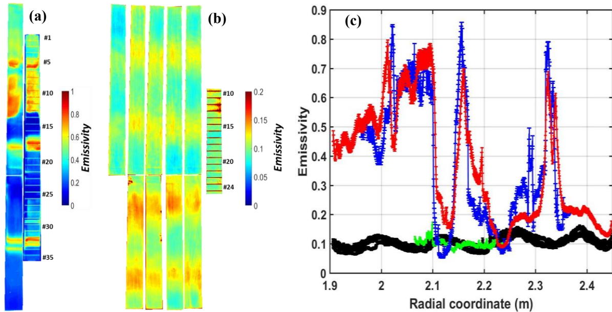
Figure 10. (a) Emissivity map after C4 for W-coated PFUs and ITER-like PFU from the location #7 of the sectors Q4B and Q3B, respectively (same location in the ripple pattern). (b) Emissivity map for non-exposed PFUs (9 W-coated PFUs and one ITER-grade PFU). (c) Emissivity distribution for (black) non-exposed W-coated PFUs, (green) non-exposed ITER-grade PFU, (red) W-coated after C4 and (blue) ITER-grade PFU after C4 extracted from figure (a).
