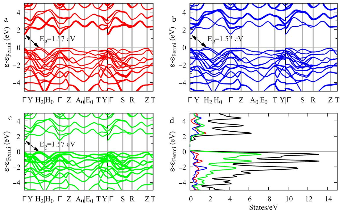
Figure 12. Band structure (a–c) and density of states (d) of \text{InGaS}_3 . The thickness of the bands is proportional to the contribution of the indium (a), gallium (b), and sulfur (c) orbitals.
