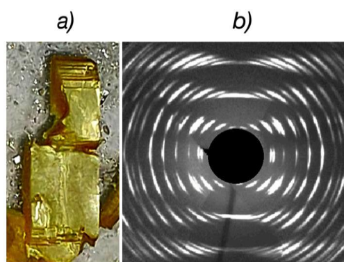
Figure 3. Crystal image (a) and XRD pattern (b) of the intercalated \text{In}_{1.2}\text{Ga}_{0.8}\text{S}_3 \cdot 0.5(\text{p-AP}) crystals.
