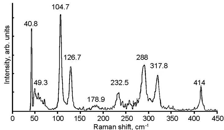
Figure 9. Raman spectrum of the GaInS 3 compound.
