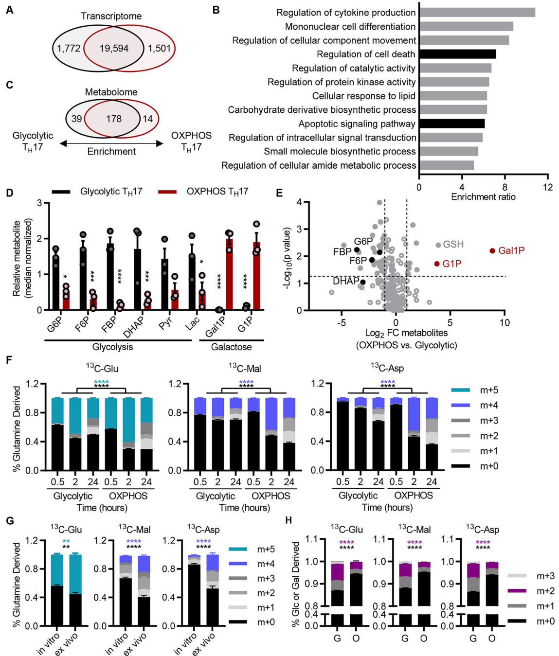
Figure 3: Transcriptomic and metabolomic profiling of OXPPOS and glycolytic TH17s. (A) Venn diagram depicting the number of differentially expressed genes ( \log_2 fold change > 0.5 , adjusted p -value < 0.05 ) between glycolytic (black) and OXPPOS (red) TH17s analyzed by RNA-seq. (B) Gene Ontology analysis of the top 500 significantly changed genes from (A). (C) Venn diagram depicting the number of differential metabolites ( \log_2 fold change > |1| , p -value < 0.1 ) between glycolytic and OXPPOS TH17s analyzed by metabolomics.
