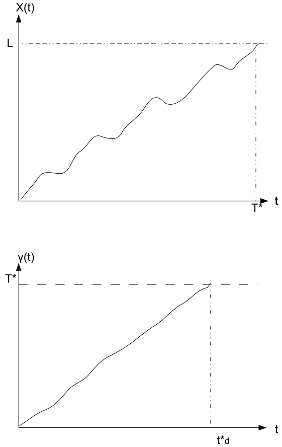
Fig. 1. First hitting time of second kind.
