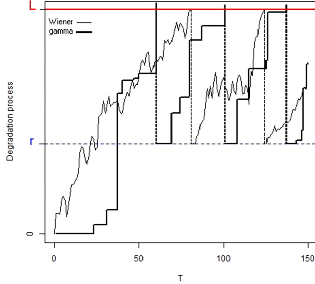
Fig. 1. A sample path of the degradation model.
