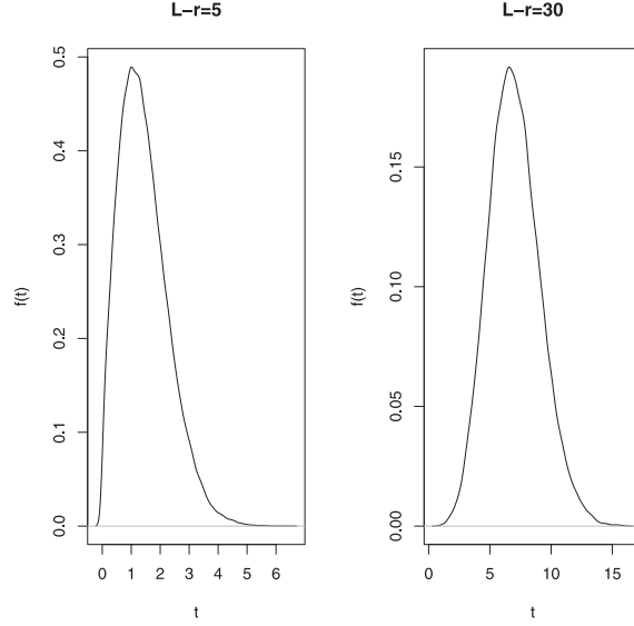
Fig. 2. Plot density functions of the first hitting times in Gamma process.
