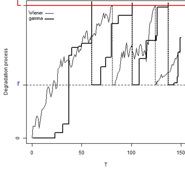
Fig. 1. A sample path of the degradation model.
