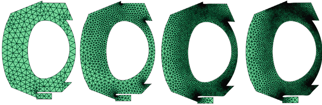
FIGURE 1 Sequence of consecutive refinements and coarsening (from left to right) starting with a initial coarse mesh of uniform size. The error estimator used to drive the process is based on the density n with the target error set at 10^{-4}
