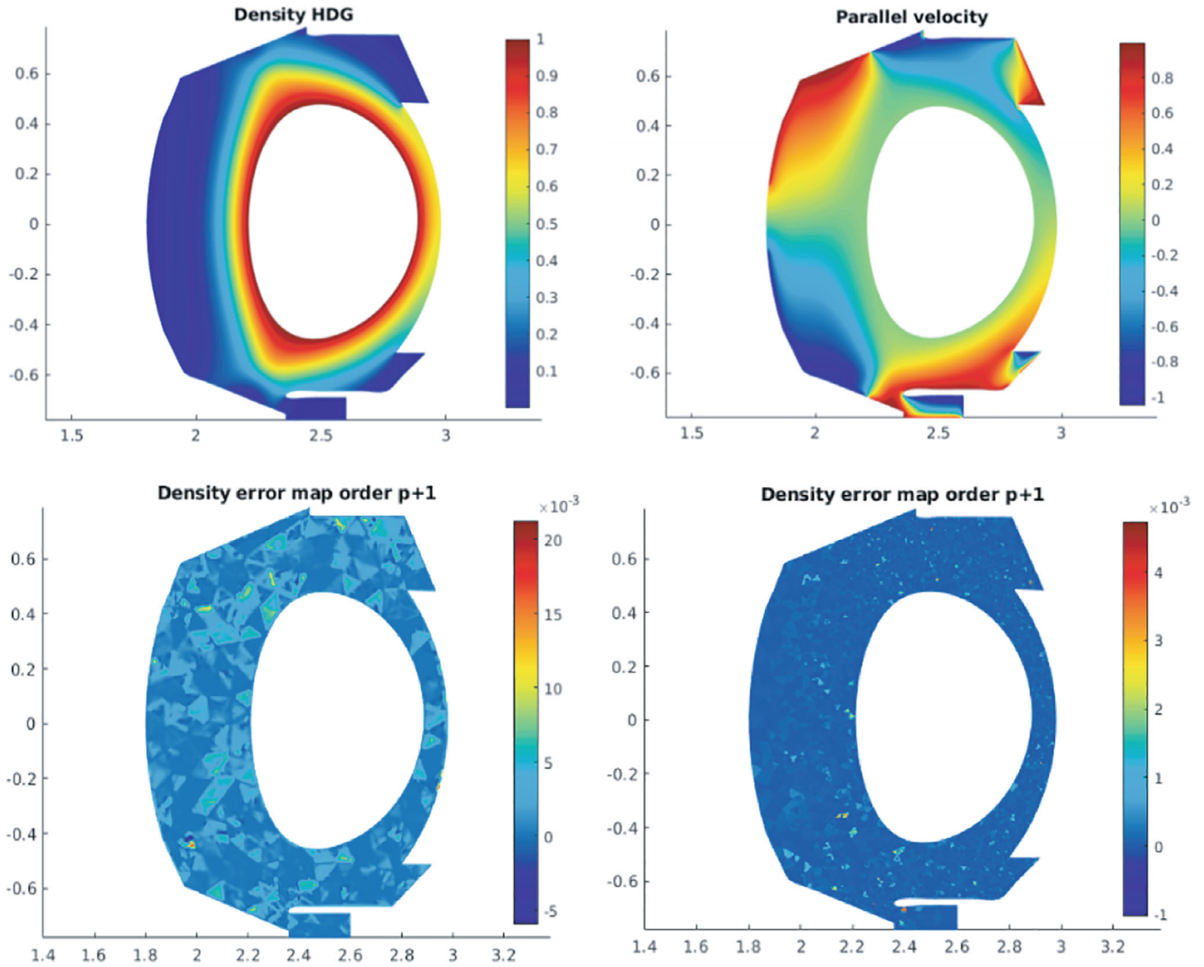
FIGURE 2 Top: solution for the density and parallel velocity at the last iteration of the adaptive process. Bottom: error map plots at the first and last iteration. The error estimator used to drive the process is based on the density n and it is projected on the higher order p + 1 = 6
