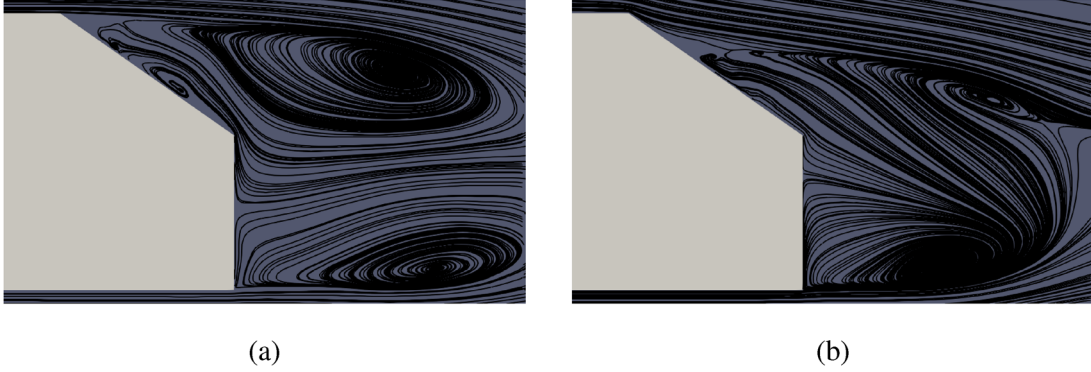
FIG. 5. Center plane time-averaged streamlines around the rear end of the Ahmed body: (a) no-slip and (b) wall-law.
