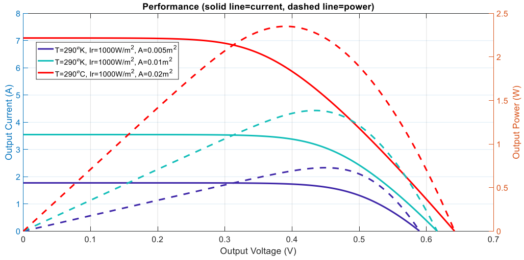
Figure 11: Evolution of the cell performance according to the variation of the surface area of (0.005m^2, 0.01m^2, 0.02m^2) . The irradiance and the ambient temperature are considered constant: 1000W/m^2 for the irradiance and 290^{\circ}K for ambient temperature.
