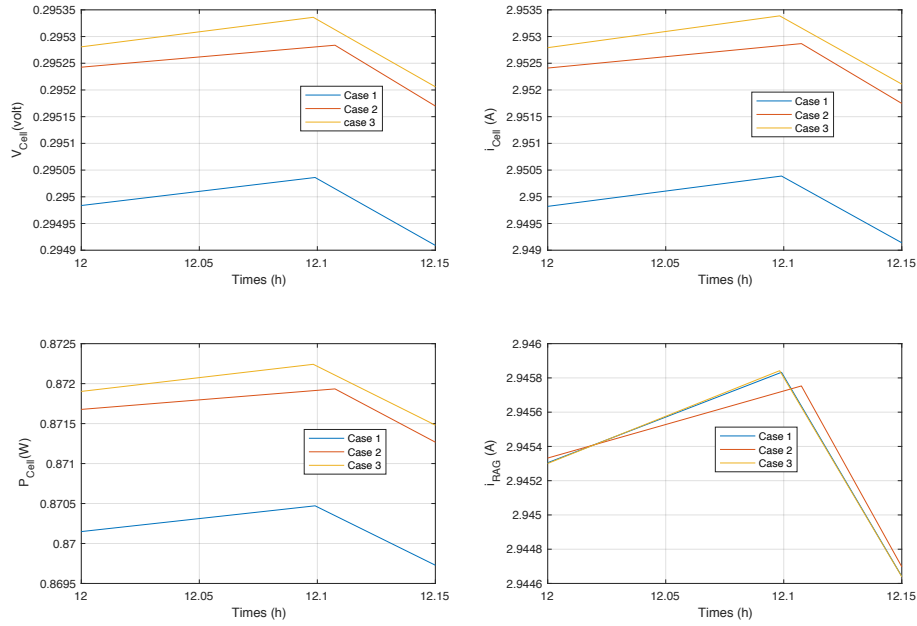
Figure 12: Evolution of the cell voltage v_{cell} and the cell current i_{cell} , the cell power P_{cell} according to the variation of v_{oc} in three cases: case 1: v_{oc} = 500mv , case 2: v_{oc} = 600mv , case 3: v_{oc} = 700mv
