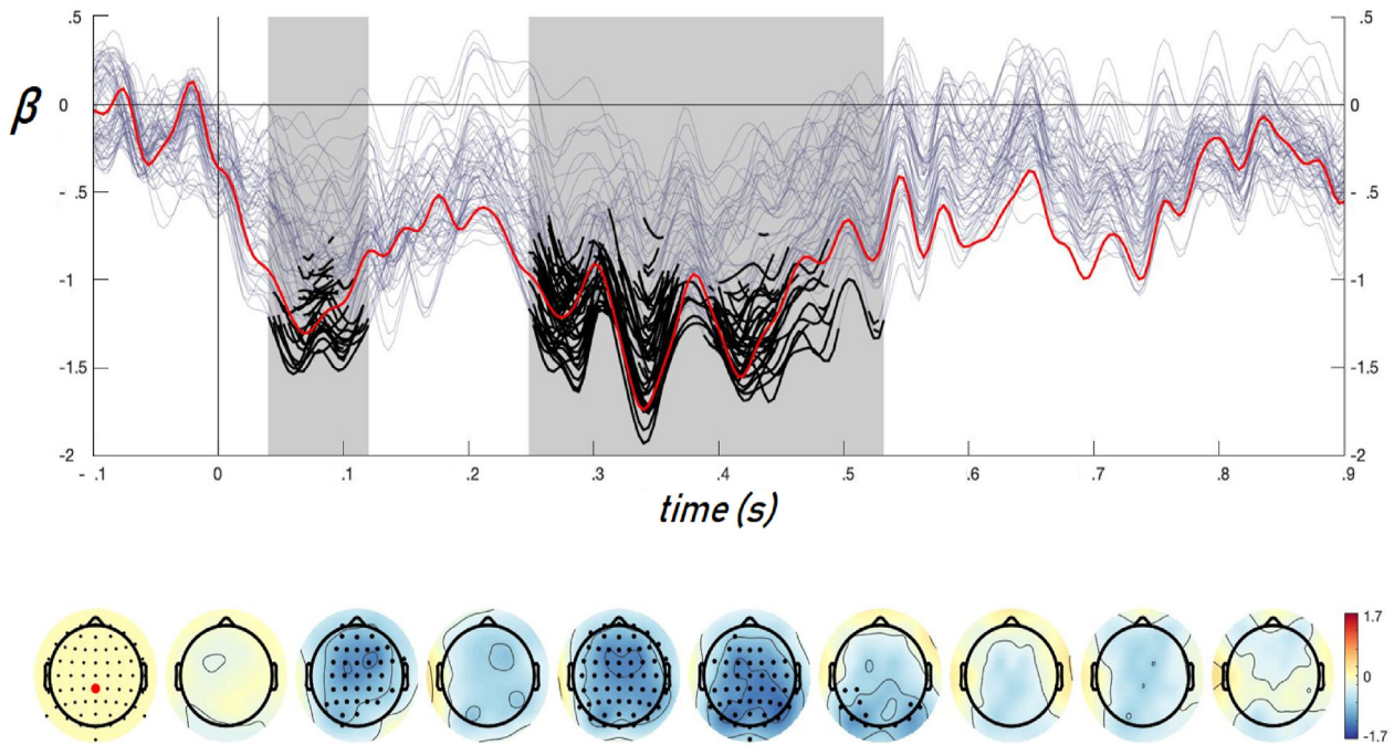
Fig. 3 – Deflection differences between the Compatible (ref.) and Incompatible condition from -0.1 to 0.9 s about the fixation. Traces in bold indicate belonging to the significant cluster. Electrodes belonging to the significant cluster are shown as points in the topography. The representative CPz electrode is plotted in red.
