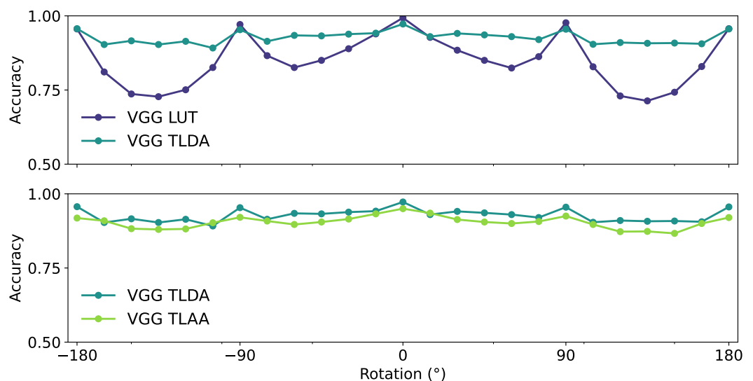
Figure 5. Average accuracy in the test dataset of the different networks for different rotations of the input image. (Top) The VGG LUT displayed with the VGG TLDA networks. (Bottom) The VGG TLA A displayed with the VGG TLDA networks. The rotation is applied around the center with an angle ranging from -180^\circ to +180^\circ .
