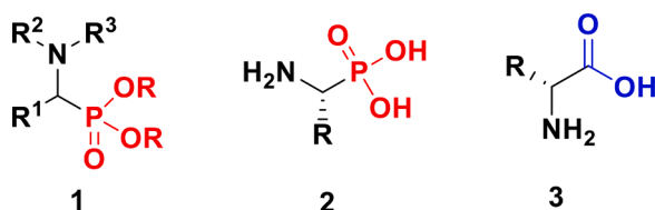
Fig. 1. Structures of α-aminophosphonate 1, α-aminophosphonic acids 2 and α-amino acids 3.
