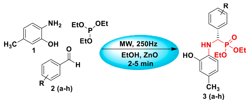
Scheme 1. Synthesis of \alpha -aminophosphonates 3a-3 h.
