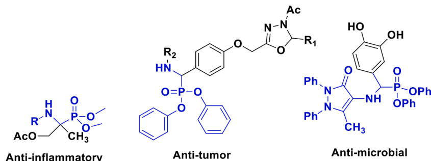
Fig. 2. Biologically active α-aminophosphonates.
