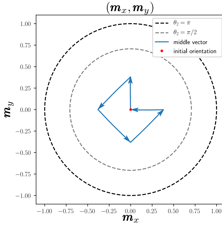
Figure 10: Projection of \mathbf{m} in the XY plane for Simulation 1 of the mono-rotor. The dashed circles indicate the possible values of (\mathbf{m}_x, \mathbf{m}_y) when \theta_2 = \pi (in black) and \theta_2 = \pi/2 (in gray).
