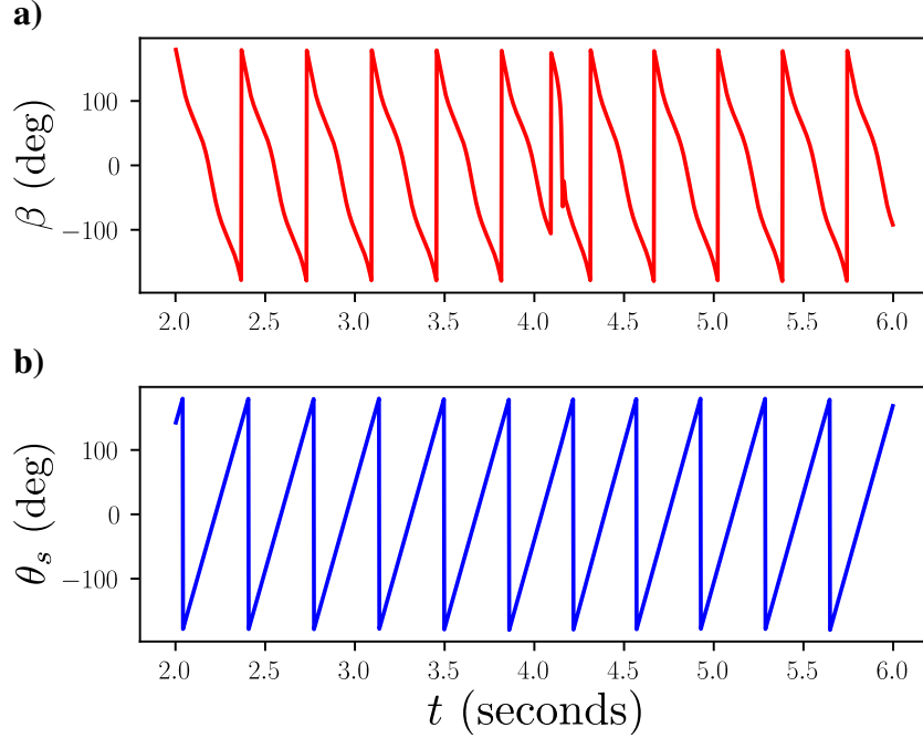
Figure 7: a) Motor phase \beta and b) robot's spin \theta_s from t = 2s to t = 6s . The swashplateless phase increases at the same rate as the spin angle, but in the inverse direction. It is also shown (at t = 4.1s ) how the motor phase suddenly shifts when the goal orientation changes.
