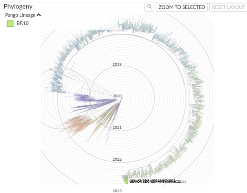
Figure 5. Position of lineage BF10 on the most recent SARS-Cov2 phylogeny (at the date of the writing of the paper): “Genomic epidemiology of SARS-CoV-2 with subsampling focused globally over the past 6 months” (Dataset: ncov, open, global, 6m; Data range: from 2019-12-17 to 2022-09-04; data form GenBank) done on nextstrain.org the 2022-09-09 ( https://nextstrain.org/ncov/open/global/6m?f_pango_lineage=BF.10 ). (top) all major clades; (bottom) focus on BF10 lineage.
