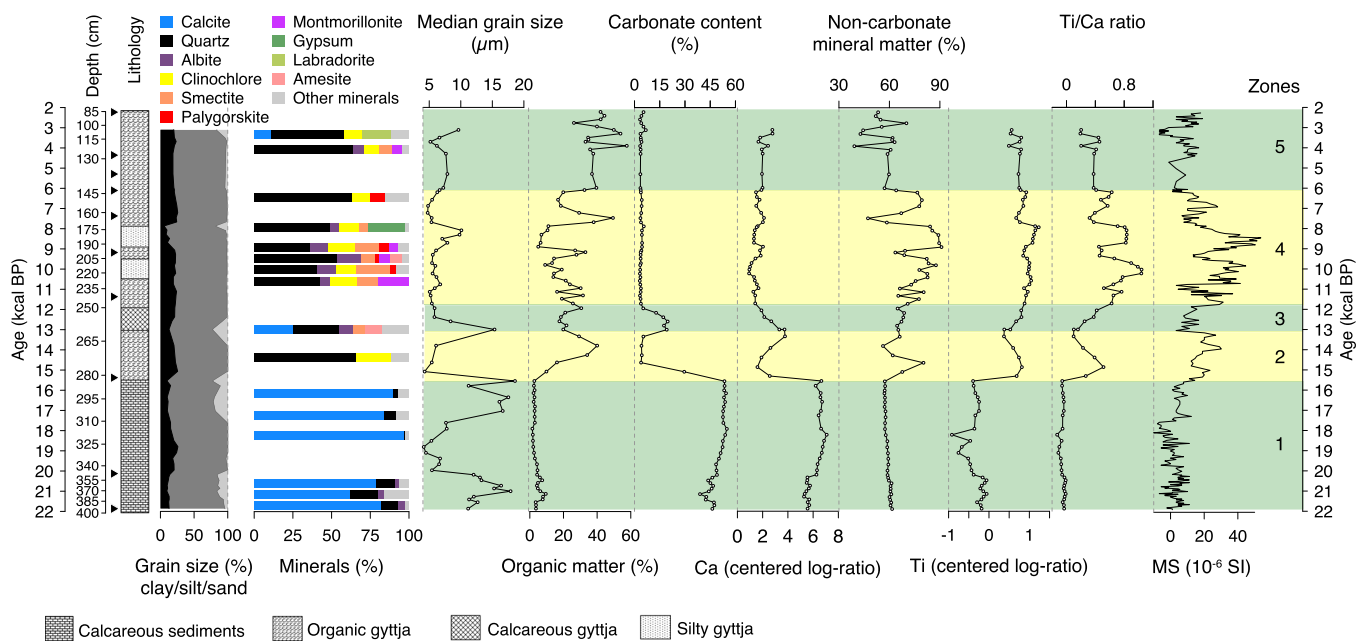
Figure 4. Lithology and downcore variations in grain size, mineral abundances, median grain size, organic matter, carbonate content, calcium (Ca), non-carbonate mineral matter, titanium (Ti), Ti/Ca ratio and magnetic susceptibility (MS). Black triangles along the lithology indicate the position of ^{14}\text{C} age controls for the sediment core. Sediment zones 1–5 are colour-shaded. [Color figure can be viewed at wileyonlinelibrary.com]
