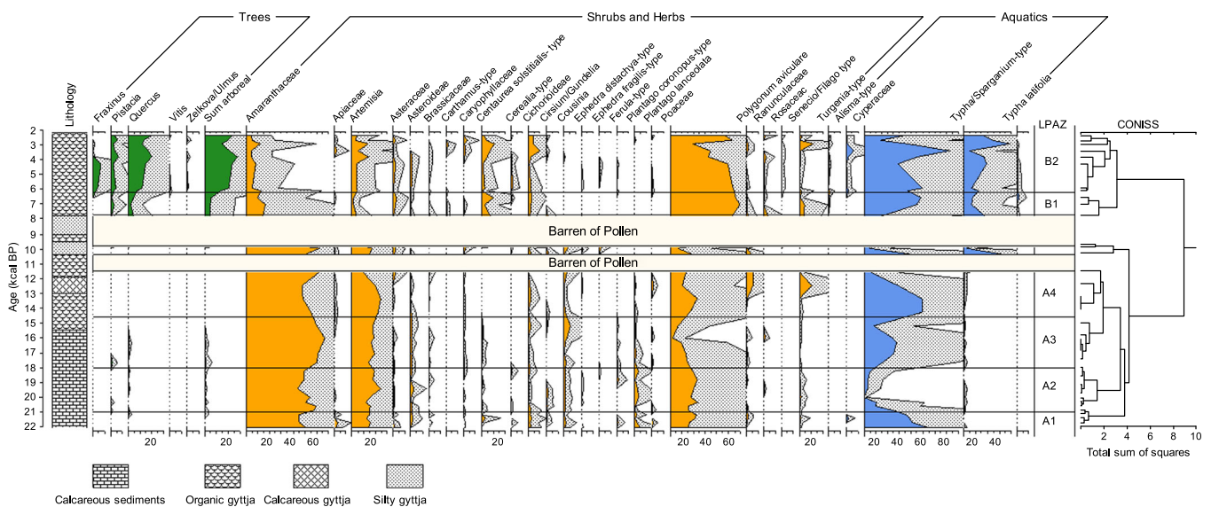
Figure 5. Pollen percentage diagram of selected taxa from the Hashilan Wetland sediment core along with local pollen assemblage zones (LPAZ) defined by CONISS. The dotted shading denotes 5× exaggeration of the original values (in %). [Color figure can be viewed at wileyonlinelibrary.com ]
