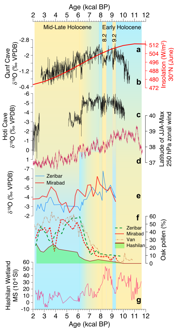
Figure 7. a. Summer insolation curve (June) for 30° N (Berger and Loutre, 1991). b. Qunf Cave stalagmite \delta^{18}\text{O} from southern Oman (Fleitmann et al., 2003), and c. Hoti Cave stalagmite \delta^{18}\text{O} from northern Oman (Fleitmann et al., 2007), a proxy for ISM rainfall variations. d. A Hovmöller plot of mean June–July–August zonal wind maximum (JJA-Max) at 250hPa (U250_max) averaged longitudinally between 30 and 60° E in the Trace experiment (Sharifi et al., 2018). e. Oxygen isotope profiles of Zeribar and Mirabad lakes (Stevens et al., 2001; Stevens et al., 2006). f. Oak pollen records for Zeribar and Mirabad lakes (van Zeist and Bottema, 1977), Lake Van (Wick et al., 2003) and Hashilan Wetland (this study). g. Magnetic susceptibility record of Hashilan Wetland (this study). Blue and yellow shadings indicate wet and dry climate intervals, respectively. 9.2: 9.2 ka event, 8.2: 8.2 ka event. [Color figure can be viewed at wileyonlinelibrary.com ]
