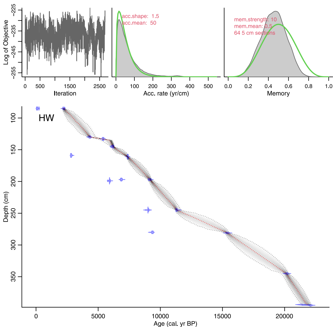
Figure 3. Bayesian age–depth model for the Hashilan sediment core. In blue: distribution of individual dates. The best model is shown by the red dotted line and the 95% probability interval by the shaded area between grey dotted lines. The upper part shows the Markov chain Monte Carlo (MCMC) iterations (left), the prior (green) and posterior (grey) distributions for the accumulation rate (middle) and memory (right). [Color figure can be viewed at wileyonlinelibrary.com ]
