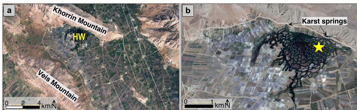
Figure 2. a. Satellite image of the Hashilan Wetland (HW) and its surrounding limestone catchment (Google Earth: 6 February 2019). b. Satellite image of the island-like surface of Hashilan Wetland with location of coring (yellow star) and karst springs (Google Earth: 14 June 2019). [Color figure can be viewed at wileyonlinelibrary.com ]
