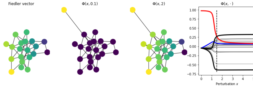
Fig. 2: From left to right: Fiedler vector of a Erdős-Renyi random graph, values are encoded from blue ( - ) to yellow ( + ); Fiedler vector of the perturbed graphs with x = 0.1 and x = 2 ; Plot where each curve corresponds to \Phi(x, i) with i fixed. In blue i = v , in red i = n + 1 and in black the vertices of the two extrema of the initial Fiedler vector. The dotted line corresponds to the value a(v) after which n + 1 is no more an extremum of \Phi(x, \cdot)
