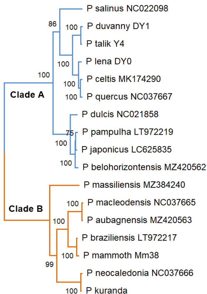
Figure 2. Neighbor-joining tree of the available pandoravirus isolates. The tree was built from 2052 gap-free sites in the multiple alignment of 17 RNA polymerases (RPB1) protein sequences using the MAFFT online facility from the Osaka University server [53]. The inclusion of the permafrost isolates confirms the ancient branching of the Pandoraviridae in two separate clades. Accession numbers are indicated following the isolate name when available.
