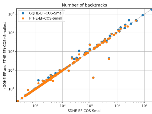
(e) # Backtrack Comparison
