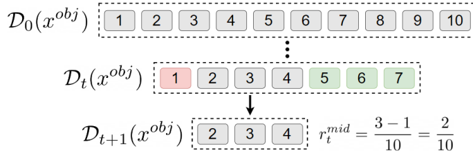
■ Figure 3 Intermediate reward when four values are pruned from the domain.
