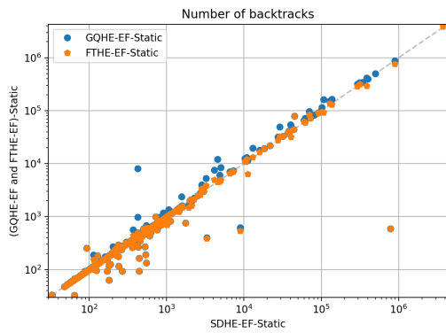
(a) # Backtrack Comparison
