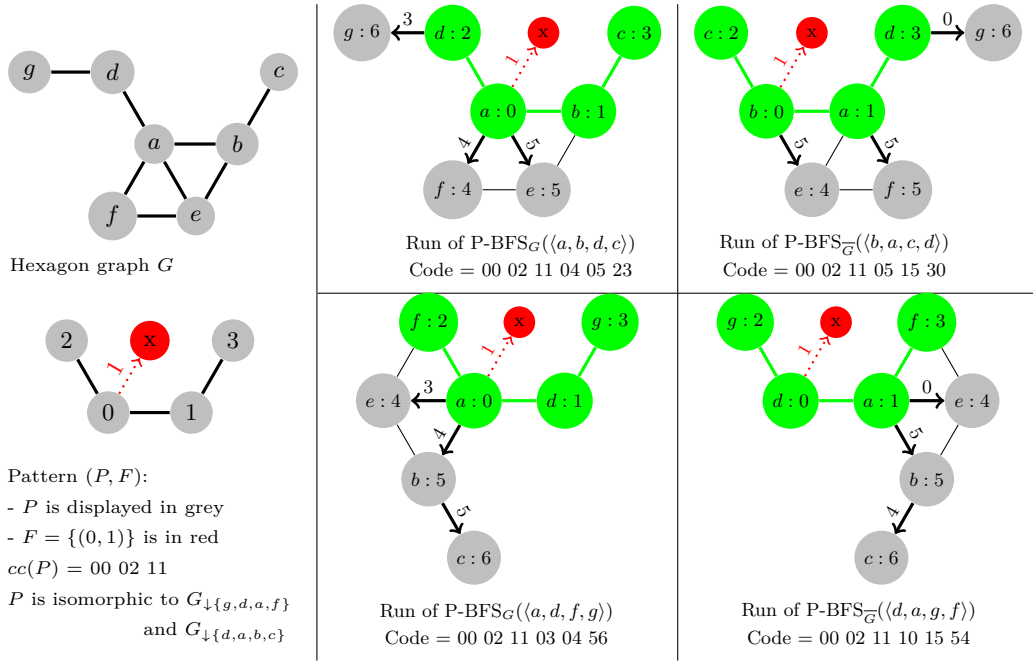
■ Figure 5 Left: Example of hexagon graph G and pattern (P, F) . Right: To compute cc_{P,F}(G) , we run P-BFS _G (resp. P-BFS _{\overline{G}} ) with the P-sequences \langle a, b, d, c \rangle and \langle a, d, f, g \rangle (resp. \langle b, a, c, d \rangle and \langle d, a, g, f \rangle ). The P-canonical code of G is cc_{P,F}(G) = 00\ 02\ 11\ 03\ 04\ 56 .
