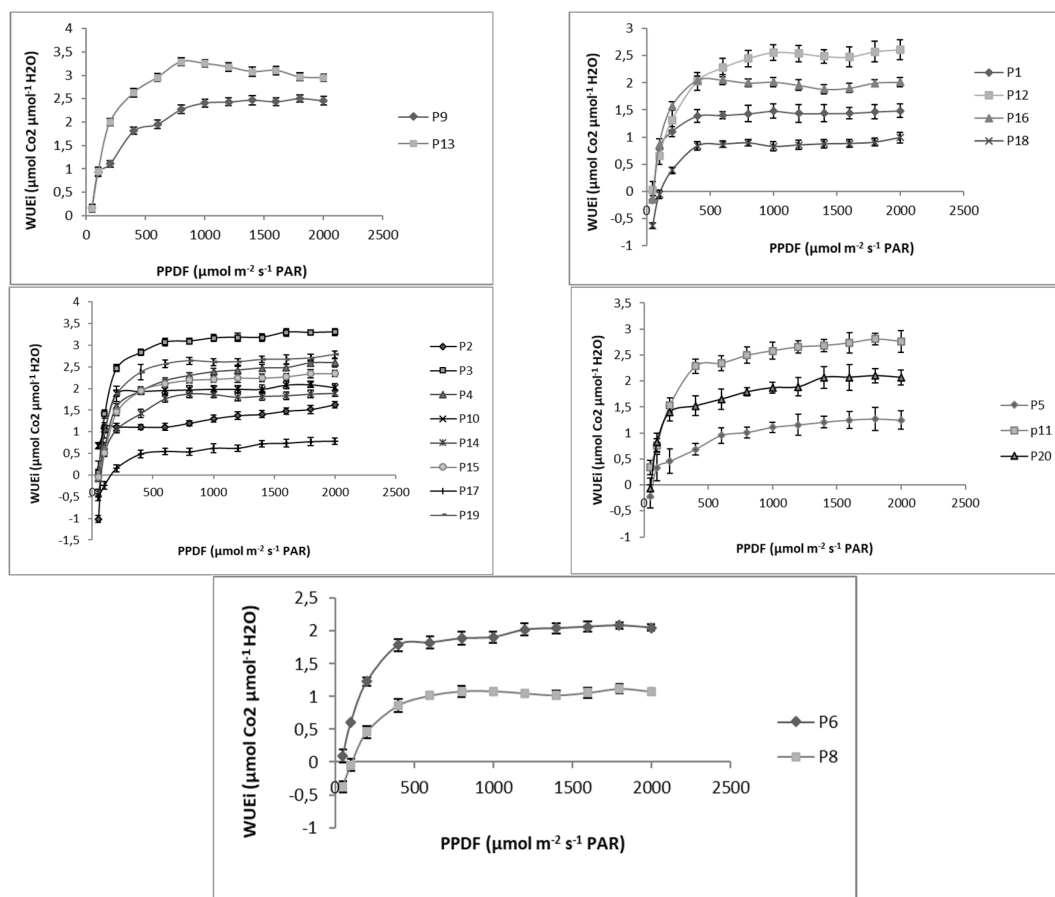
Figure 4. Response of gas exchange to light: instantaneous water use efficiency (WUEi) as a function of PPDF in an atmosphere of 400 ppm CO 2 and 25 °C Values are means \pm SE of at least three independent measurements.
