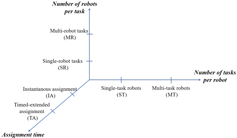
Fig. 1: MRTA problems classification.
