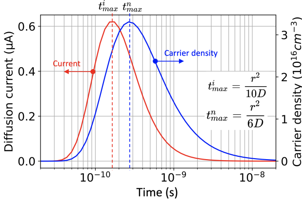
FIG. 2. Time evolution of the carrier density and the diffusion current evaluated from Eqs. (3) and (6), respectively, for a distance r = 1.5 \mu\text{m} from a point charge source Q = qn_0 . Simulation parameters are: n_0 = 1.52 \times 10^6 electrons, D = 13.78 \text{ cm}^2\text{s}^{-1} and A_S = 0.0323 \mu\text{m}^2 .
