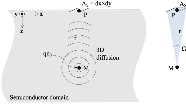
FIG. 1. Schematic illustration of the diffusion from a point charge and the collection by a small contact of surface A_S .
