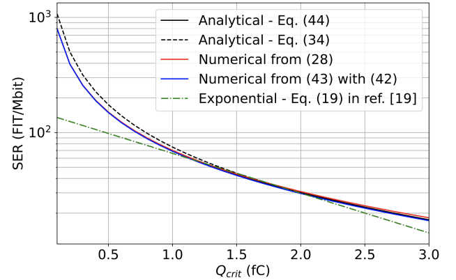
FIG. 8. SER versus Q_{crit} computed from analytical Eqs. (34) and (44), from the numerical solving of Eq. (28), of Eq. (43) considering collection velocity given by Eq. (42) and from an exponential approximation (Eq. (19) in ref 19 ) close to the empirical expression proposed by Hazucha and Svensson 20 . Simulation parameters are: A_S = 0.25 \mu\text{m}^2 , L = 2 \mu\text{m} , N = 1.38 \times 10^6 , D = 61 \text{ cm}^2 \text{ s}^{-1} , F = 10^{-3} \text{ cm}^{-2} \text{ h}^{-1} and v_{col} = 3.5 \times 10^5 \text{ cm s}^{-1} for Eq. (19) in ref. 19
