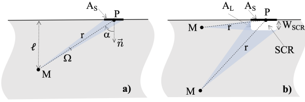
FIG. 3. Schematic illustrations of collecting contacts: a) an ideal planar contact of surface A_S and b) a “real” contact in CMOS circuits consisting in a reversely-biased junction with a layout surface A_S and a lateral surface A_L due to the depth extension ( W_{SCR} ) of the space charge region (SCR).
