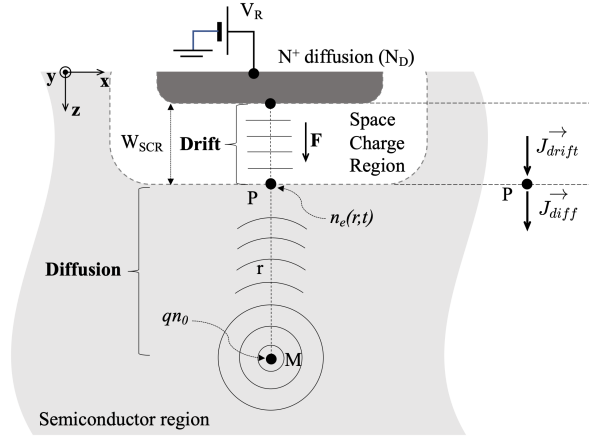
FIG. 9. Schematic illustration of the diffusion from a point charge and the collection by a reversely-biased N^+P junction.
