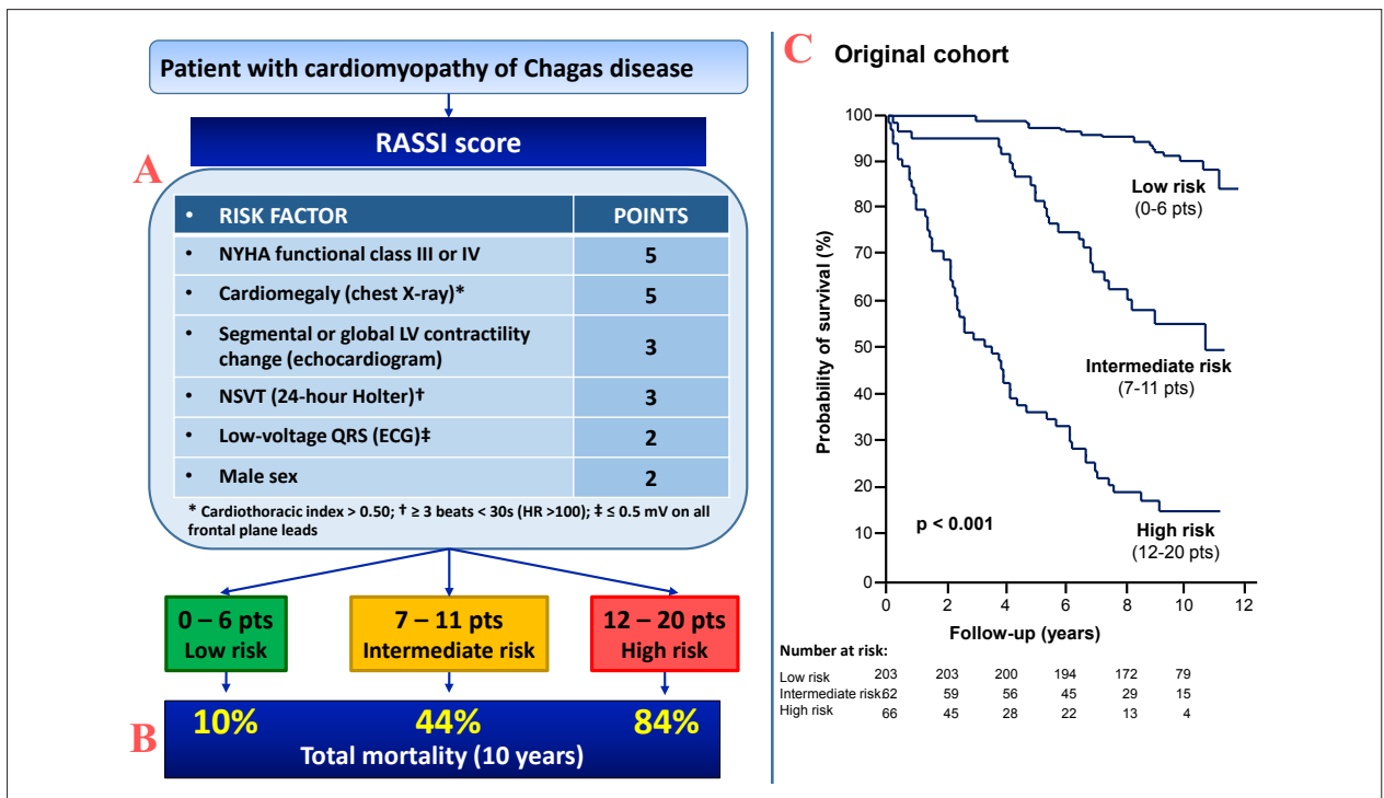
Figure 7.2 – RASSI score. (A) Risk markers and respective points; (B) Total mortality in 10 years in the low-, intermediate-, and high-risk subgroups; (C) Kaplan-Meier actuarial curves. pts: points, NSVT: Nonsustained ventricular tachycardia.
