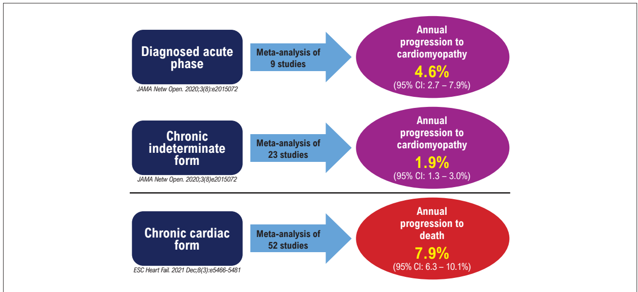
Figure 7.1 – Annual progression rate of Chagas disease (diagnosed acute phase and chronic indeterminate form) to cardiomyopathy and from chronic cardiac form to death.
