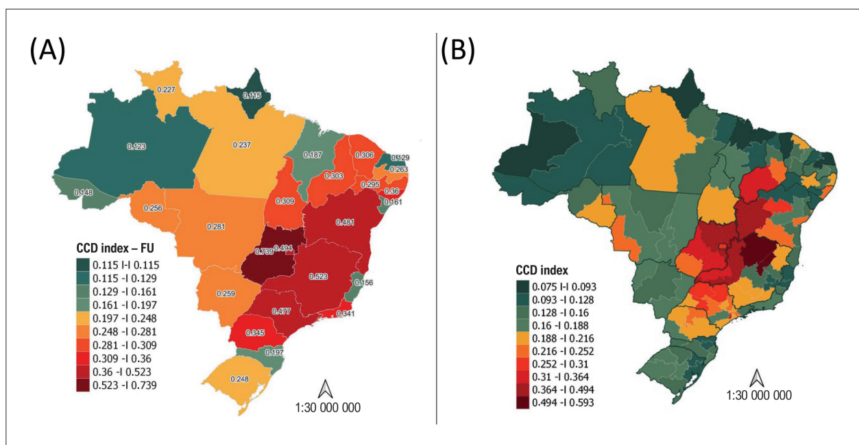
Figure 2.1 – Spatial distribution of chronic Chagas disease (CCD) vulnerability index according to the federative units (FU) and Distrito Federal (A) and health macroregions (B). Source: CGZV/Deidt/SVS
