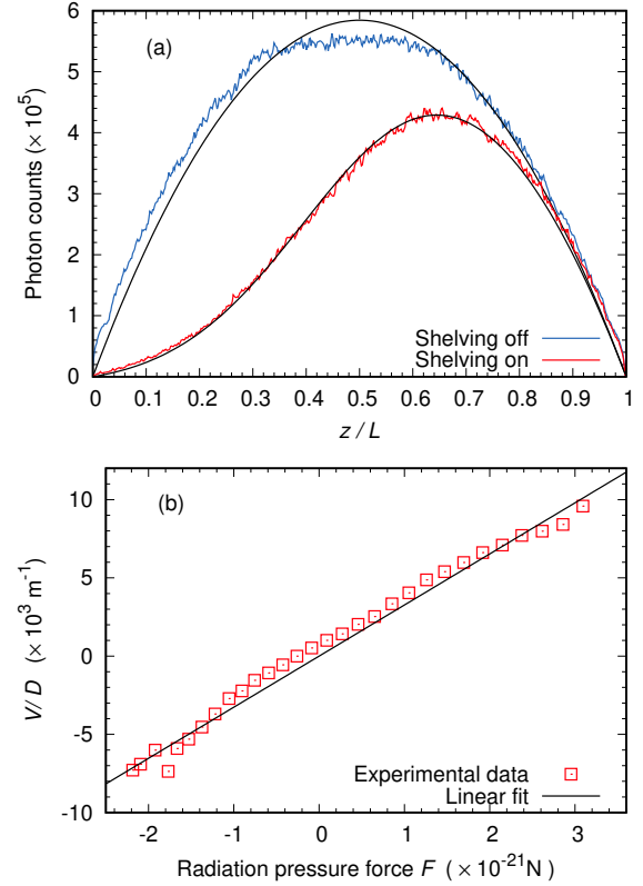
FIG. 3. Panel (a) : data analysis of a picture like shown in Fig 1, for a cloud made of 1240 \pm 60 ions with total length L = 289 \pm 7 \mu\text{m} , and a measurement time of 1 s. Blue curve : number of collected photons I(z) , as a function of the relative coordinate z/L along the cloud symmetry axis, in the absence of shelving, when all particles are “bright”. The black line is the best fit with a parabolic profile, which is expected because the projected density of ions is just proportional to the transversal section of the cloud, Eq. (21). Red curve : number of collected photons I(z) , as a function of the relative coordinate z/L , in the case where part of the ions are shelved in a metastable state, so that they do not scatter photons. The black curve is a fit which obeys Eq. (22), taking into account the scaling factor given by the previous fit. Panel (b) shows the value of V/D , obtained from this fit, for several signal profiles I(z) obtained with different values of the effective pressure force F .
