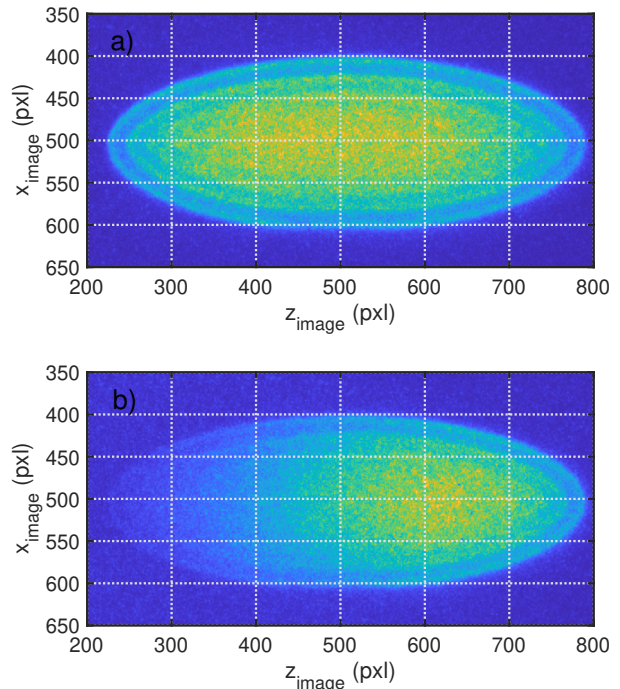
FIG. 1. (a) Picture of the laser induced fluorescence of a trapped ion cloud made of 1240 \pm 50 \text{Ca}^+ ions. Given an optical magnification of 12.6 \pm 0.3 and a pixel size of 13 \mu\text{m} , the scale of the picture in pxl is very close to the scale of the cloud in \mu\text{m} . The cloud dimensions are : R = 107(\pm 2)\mu\text{m} for the largest radius and L = 576(\pm 14)\mu\text{m} for the total length. (b) : same cloud with an extra laser admitted, propagating toward z > 0 in real space and on the picture, this laser is shelving part of the ions in a metastable dark state.
