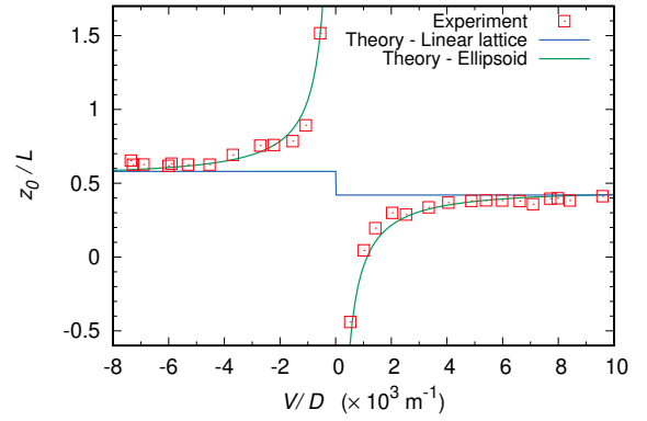
FIG. 5. Transition front coordinate z_0/L as a function of the drift. Red squares represent the values measured in experiments (i.e., from the fits of density profiles, as shown in Fig. 4a). The blue solid line shows the approximate estimate provided by Eq. (18) for the linear-lattice geometry. The green solid line is computed taking into account the ellipsoidal geometry, see Eq. (23).
