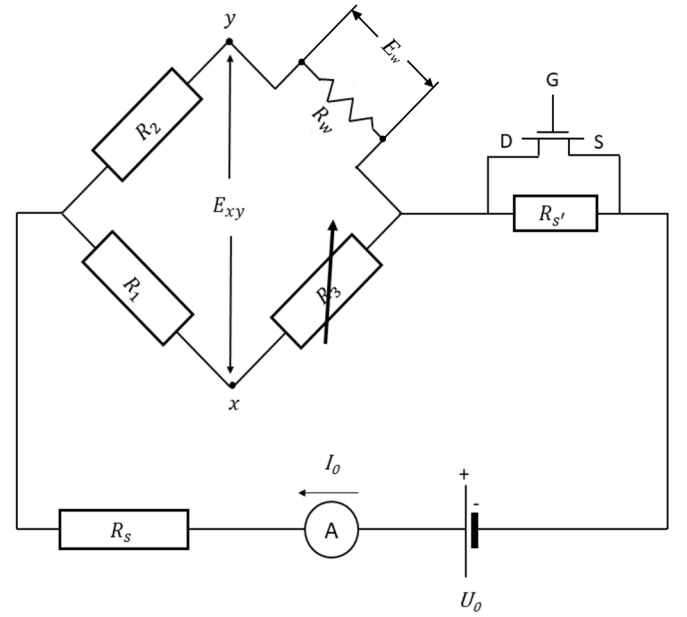
Fig. 1 Sketch of the constant current anemometer system.
