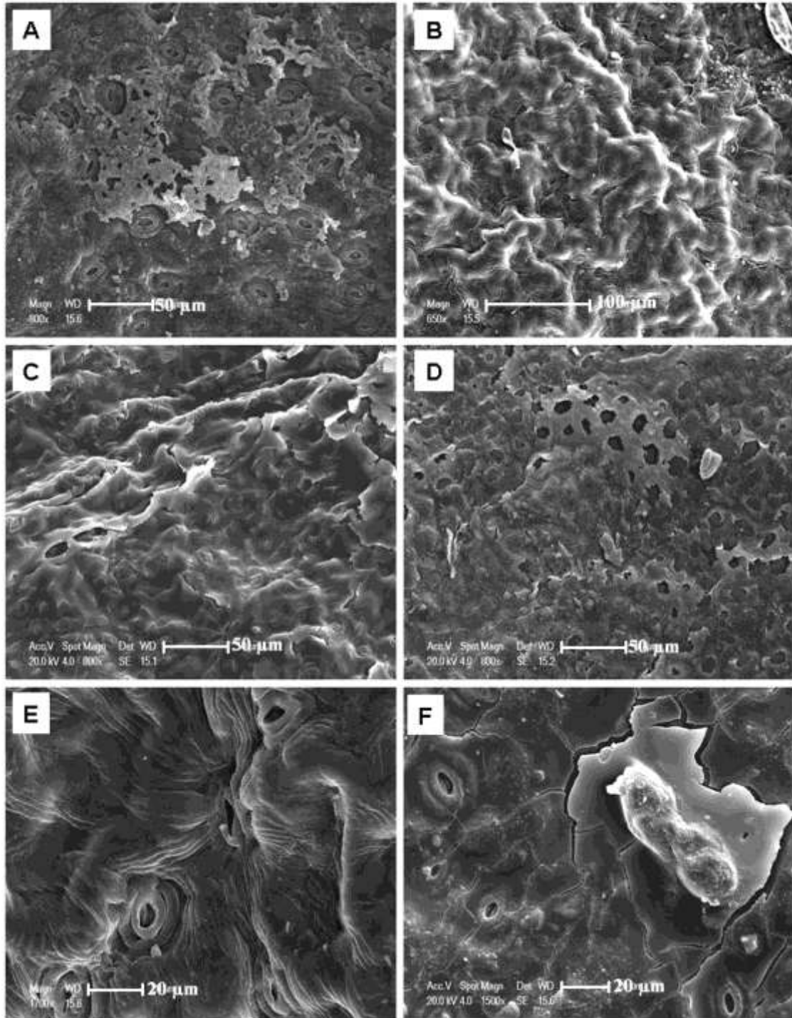
Figure 2.- SEM micrographs of abaxial and adaxial leaf surfaces of P. lentiscus from different populations showing waxes' features. (A-B) granulate and anomorphous deposits in thin layers of waxes over the epidermis surface in Boumerdes site (A and E) abaxial face, (B) adaxial face. Glossy aspect of the wax layer on the abaxial face in Senalba site (C), granulate deposits on the adaxial face in Hamdania site (D), wax crust on the adaxial leaf surface (F).
