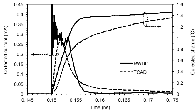
Fig. 14. Current and charge collected by an isolated OFF-state NMOS transistor (designed in 65 nm CMOS technology) after a 5 MeV alpha particle strike computed by TCAD and by the RWDD model. (After Autran et al. [78], © Elsevier 2014.)
