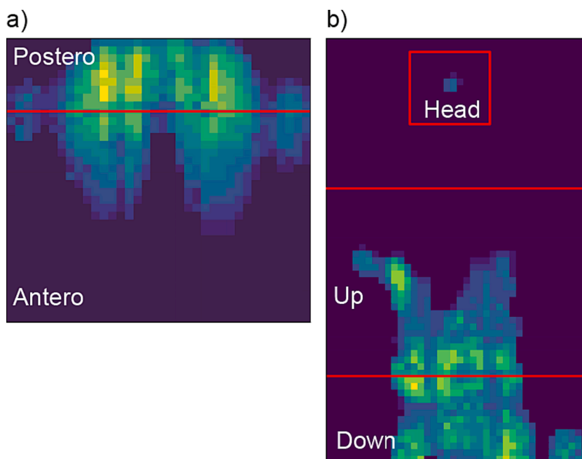
Fig. 2. Sensor mats for the seat cushion (a; 36 \times 36 cells) and the backrest (b; 40 \times 64 cells). Red lines illustrate the demarcation between zones. Seat cushion mat was sliced into 2 zones: posterior and anterior. Backrest mat was sliced into three zones: head, upper and lower back. (For interpretation of the references to colour in this figure legend, the reader is referred to the web version of this article.)
