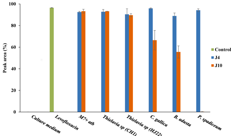
Fig. 2. Time-course data on levofloxacin degradation by Thielavia sp. CH1 , Thielavia sp. HJ22 , Corioliopsis gallica (Ben Ayed et al., 2022a), P. spadicum , and B. adusta at day 4 (here, in blue) and day 10 (orange) of culture. Culture medium alone (M7), levofloxacin at 50 mg L -1 in water (green), and culture medium (M7) with 50 mg L -1 levofloxacin (on day 4 and day 10) were used as controls. Each datapoint is the mean ± standard deviation of triplicate experiments.
