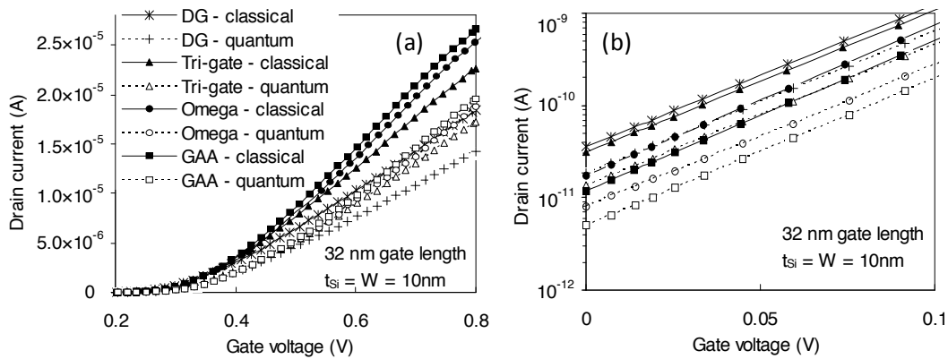
Fig. 22. Drain current I_D(V_G) characteristics in classical and quantum mechanical cases for 32 nm DG, Tri-gate, \Omega -Gate and GAA architectures ( V_D = 0.8 V): (a) the above threshold regime; (b) zoom on the subthreshold characteristics. After [100]. © 2007 Institute of Electrical and Electronics Engineers Inc., reproduced with permission.
