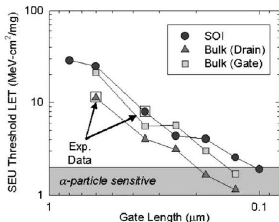
Fig. 35. Simulated LET threshold versus gate length trend for 6T SRAM cells in a bulk Silicon technology and a partially depleted SOI technology with body ties. The simulated devices are fully scaled (all parameters, gate length, supply voltage, doping level, etc., have been scaled). Predictions for the 0.6- \mu\text{m} and 0.35- \mu\text{m} technology nodes were validated against experimental data from Sandia fabricated technologies. After Dodd [15]. © 2005 Institute of Electrical and Electronics Engineers Inc., reproduced with permission.
